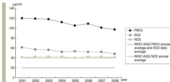
Figure 1. Ambient air pollution levels in 31 provincial capitals of China ( \mu\text{g}/\text{m}^3 , 2001–2008) - (Kan et al. , 2012).
